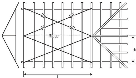
(a) Roof length "L" ≥ half span "h" of the roof truss
