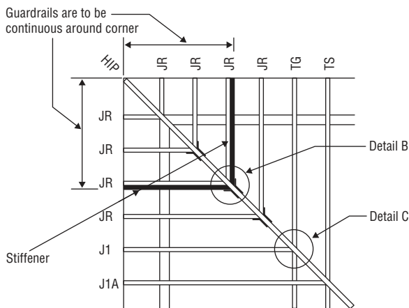
Figure 4. Truss fixings
